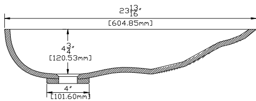
SIDE CROSS-SECTION
